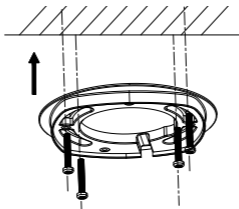
Figure 2-6 Install the Mounting Base
