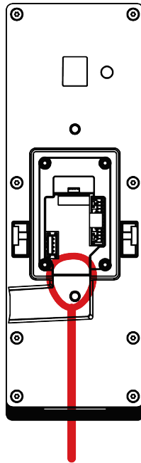
Figure 2-5 Apply silicone sealant
